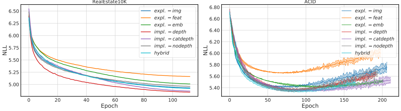
Figure 10. Negative log-likelihood over the course of training on RealEstate10K (left) and ACID (right). Implicit variants achieve the best results, see Sec. 4.1 for a discussion.
