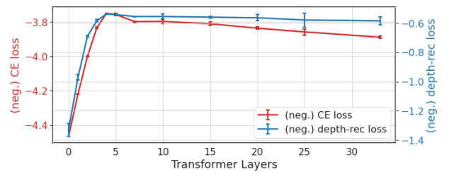
Figure 7. Minimal validation loss and reconstruction quality of depth predictions obtained from linear probing as a function of different transformer layers. The probed variant is impl.-nodepth .
